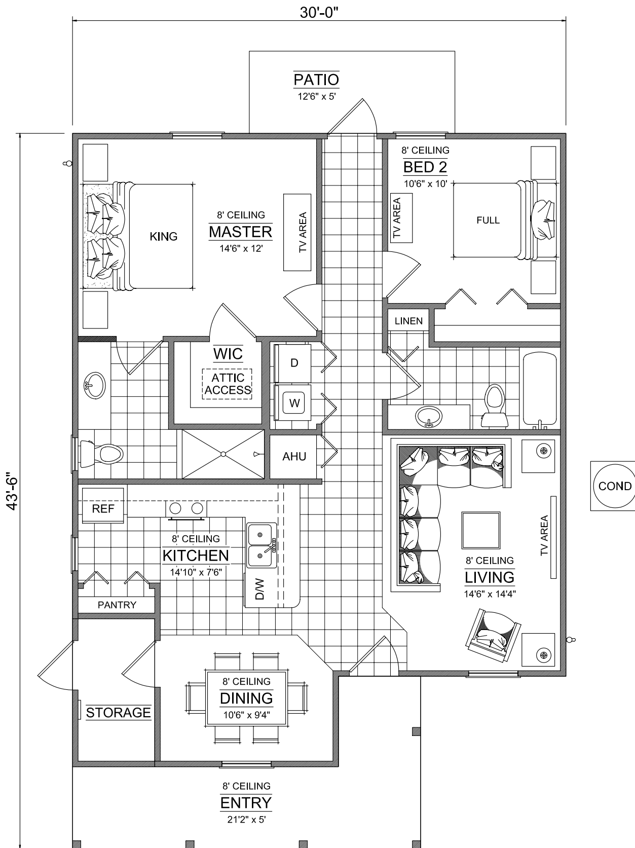
FLOOR PLAN
