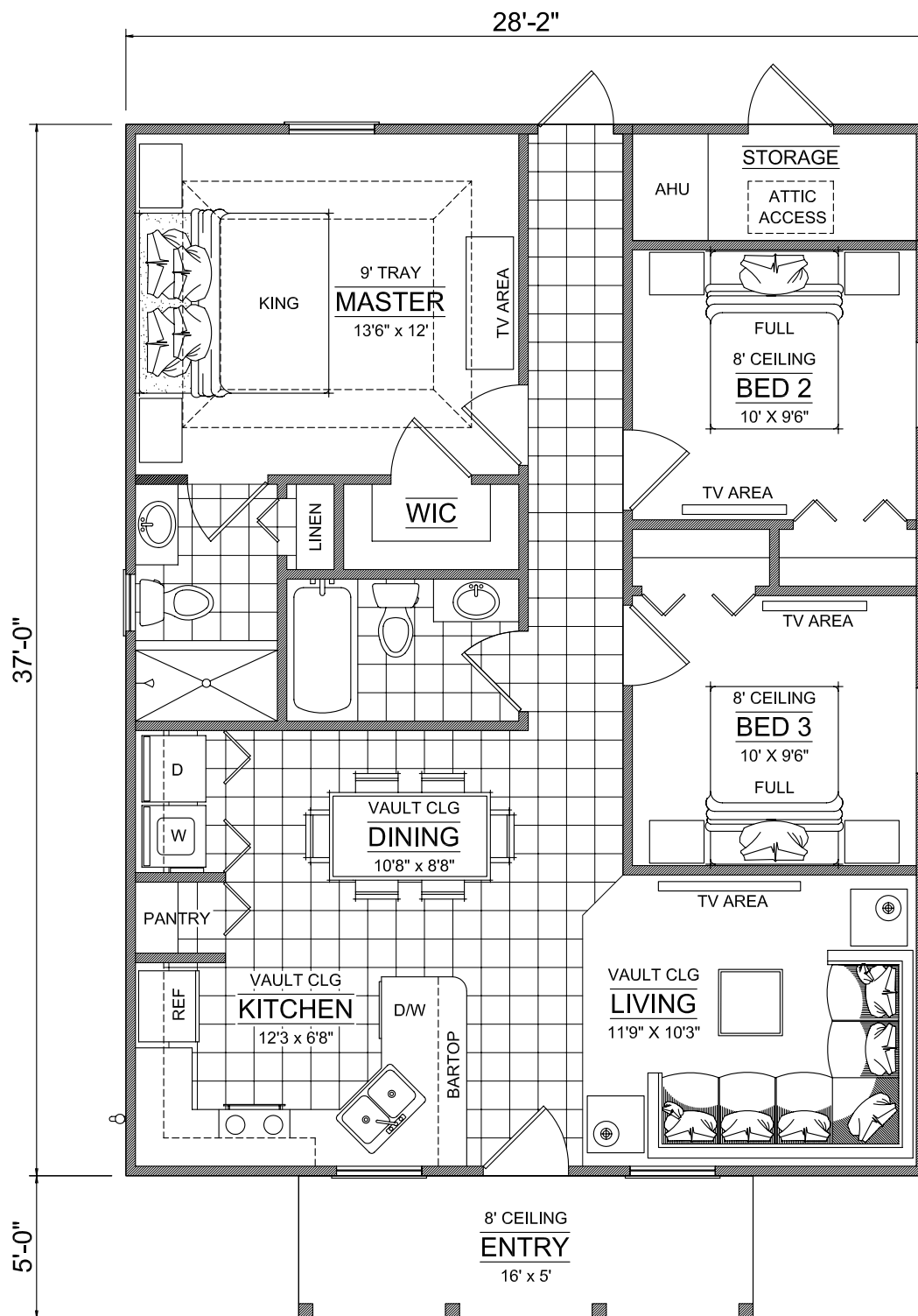
FLOOR PLAN
