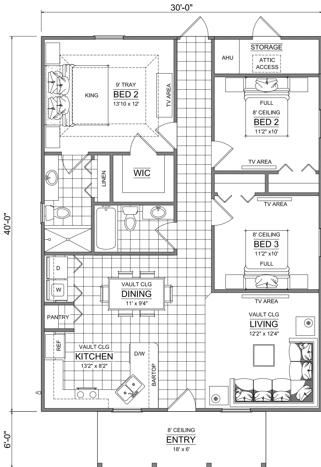
FLOOR PLAN
