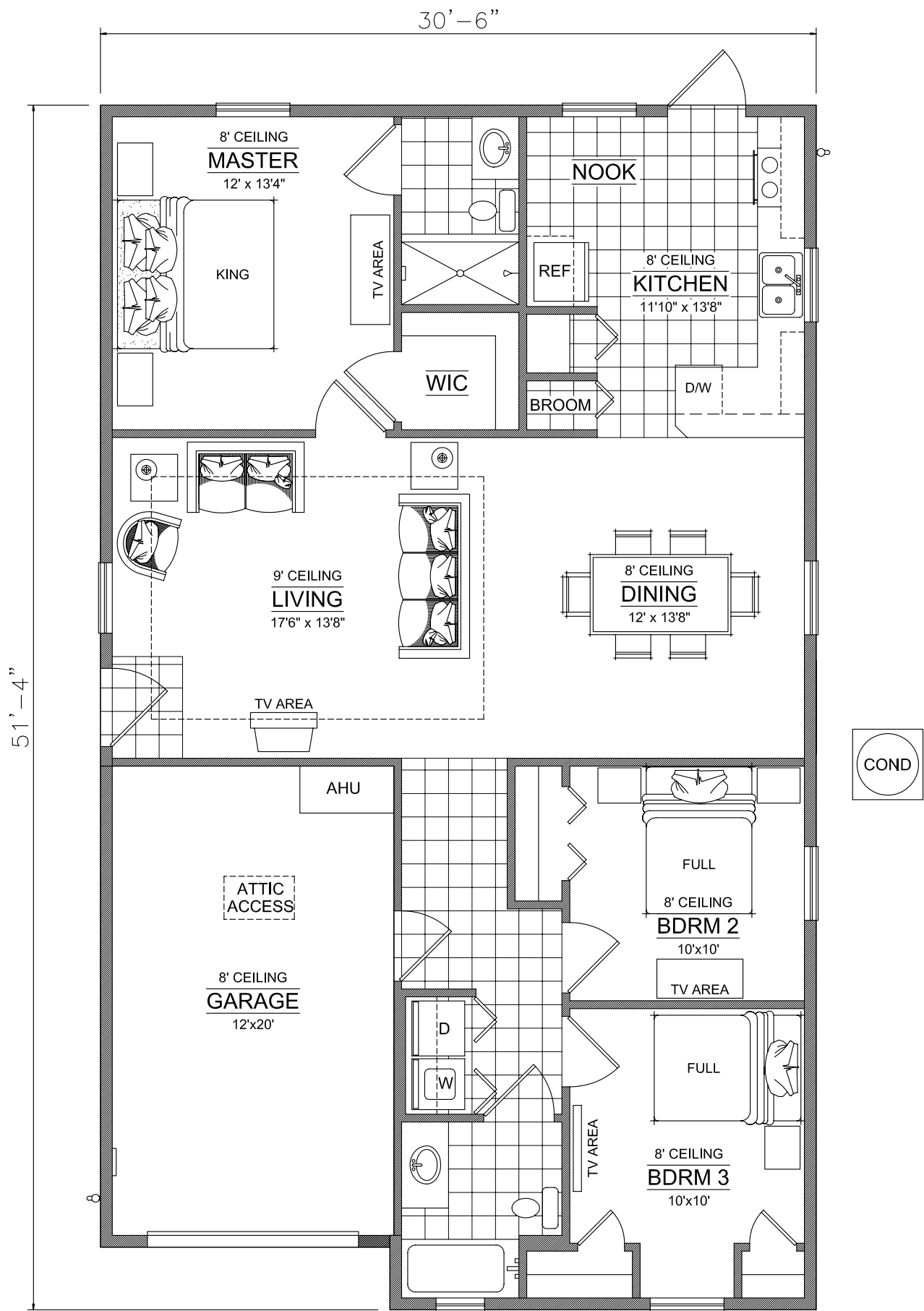
FLOOR PLAN
